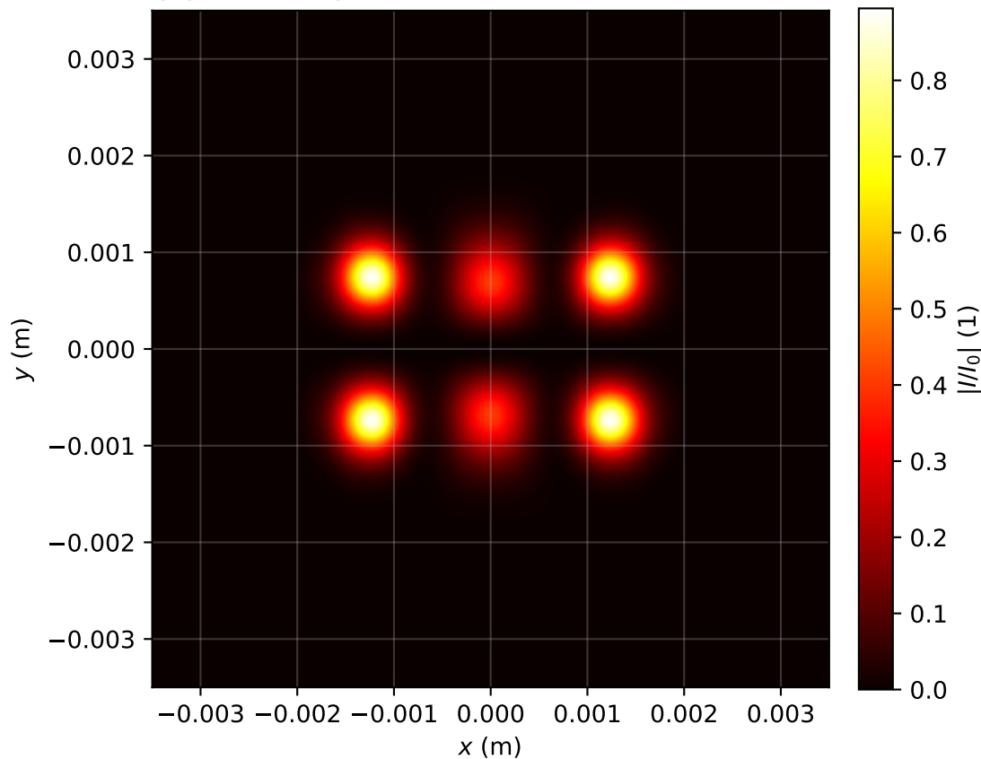
Intensity profile I(x, y, z = 2.388)/I_0 , P_{in}=3.0P_{cr} , artificial time
